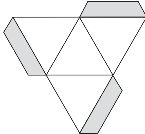
Tetrahedron
